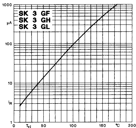
Fig. 13 Reverse current vs. junction temperature
