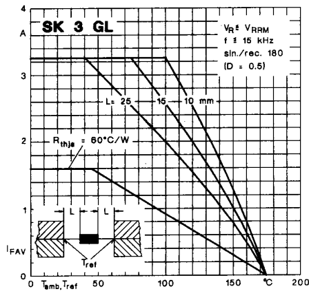
Fig. 12 c Rated forward current vs. temperature
