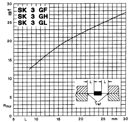
Fig. 14 Thermal resistance vs. lead length
