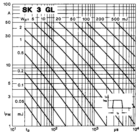
Fig. 4 c Forward energy dissipation, rectangular
