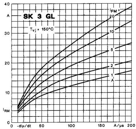
Fig. 6 c Peak reverse recovery current
