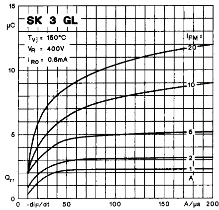
Fig. 5 c Recovered charge
