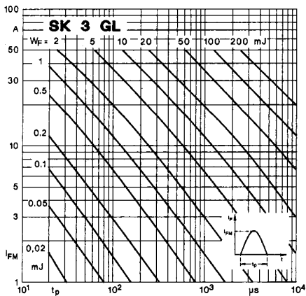
Fig. 2 c Forward energy dissipation, sinusoidal
