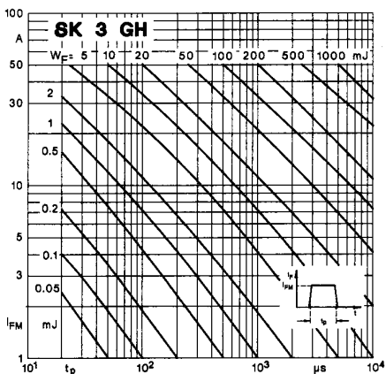
Fig. 4 b Forward energy dissipation, rectangular
