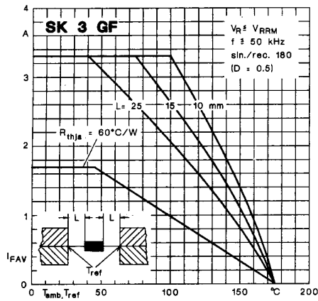
Fig. 12 a Rated forward current vs. temperature
