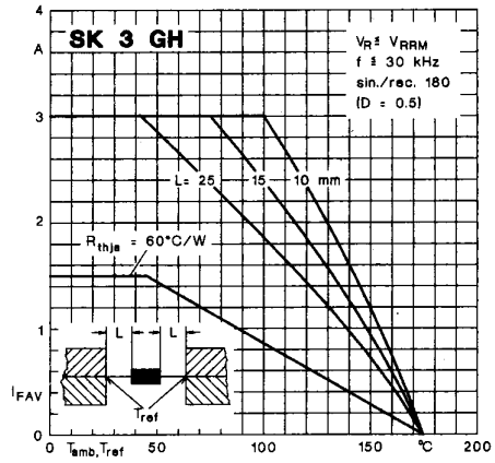
Fig. 12 b Rated forward current vs. temperature
