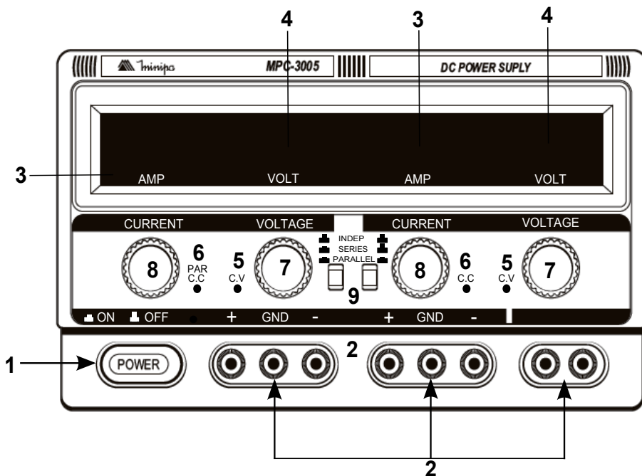
Figura 1 – Painel Frontal Fontes MPC-3003 e MPC-3005
