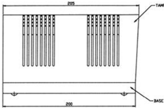
PAINEL TRASEIRO
