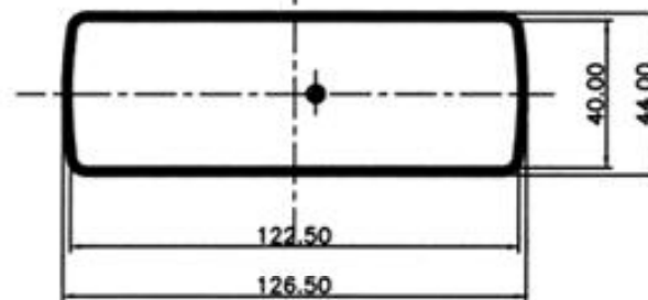
TAMPA
