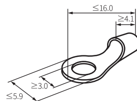
Round crimp terminal
